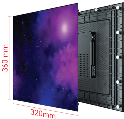
Front & Back Side LED Module
